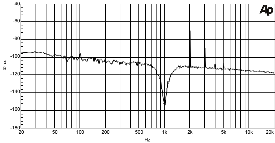
Graph 3: Distortion spectrum
